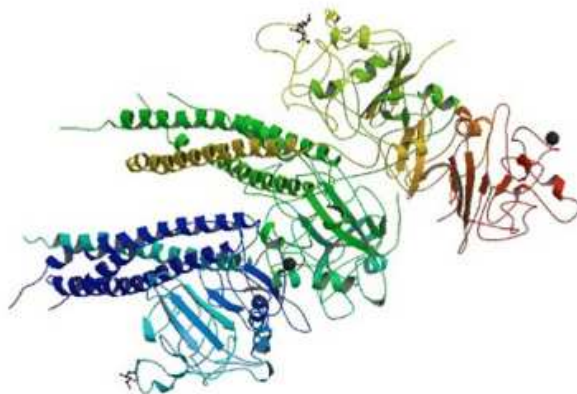
Figure 10.1: Fibrinogen
