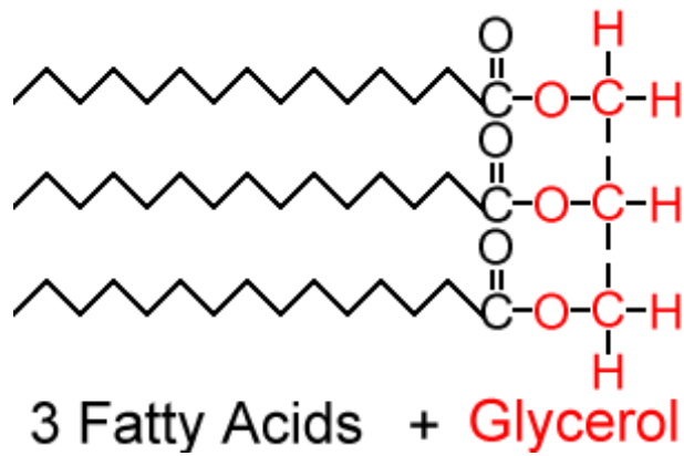
Figure 7.6: A triglyceride molecule
