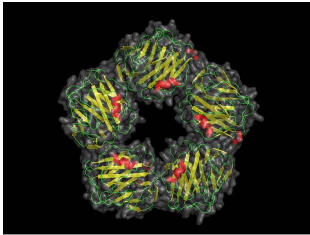
Figure 7.8: The C-reactive protein molecule.
